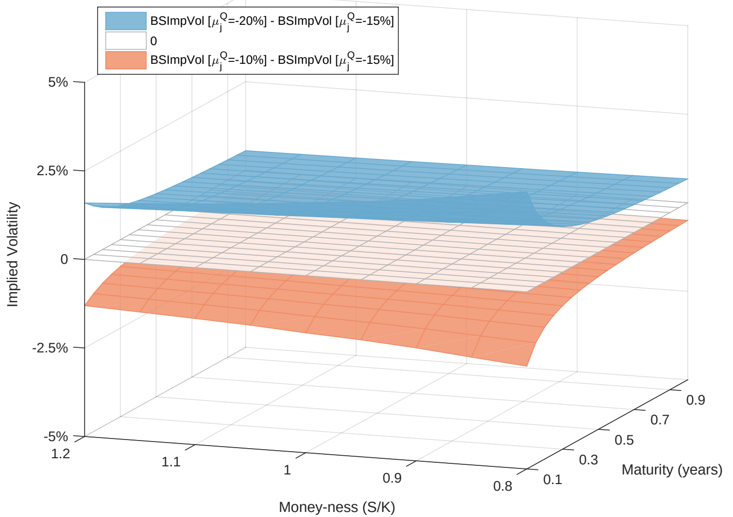
Impact of \mu_j^Q on option prices
